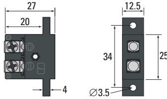
Type J IEC illustrated (R27J-I). Recommended cutout: 13mm x 26mm
