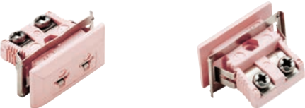
Type N IEC illustrated (F29SN-I). Recommended cutout: 8mm x 16.5mm
